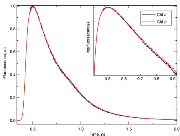
Fig. 2. Fluorescence decay curves of PSII membranes with 2.35 LHCII trimers per RC, measured at 13 °C. The black trace (Chl a ) corresponds to excitation at 420 nm and the fitted decay times and relative amplitude are 74 ps (41.7 %), 175 ps (51.0 %), 377 ps (7.1%) and 2.2 ns (0.1%). The red trace (Chl b ) corresponds to excitation at 484 nm detection and the fitted decay times and relative amplitude are: 81.3 ps (41.4%), 179 (51.9%), 380 ps (6.6%) and 1.8 ns (0.1%). Fluorescence is detected with a 688 nm band-pass filter. The inset focuses on the first part of the decay and the fluorescence is represented on a log scale.
